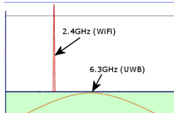
Figure 4 - WiFi v UWB Power / Bandwidth
