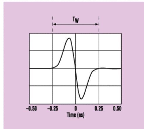
2. The basic pulse transmitted by a UWB transmitter is called a monocycle. It's not one cycle of a sinewave, but a unique pulse shaped by a Gaussian filter.
